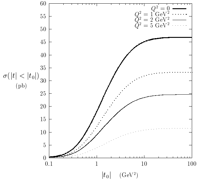
Fig. 4. Total cross section for the process \gamma^* p \rightarrow \eta_C p integrated over the region 0 < |t| < |t_0| as a function of |t_0|
