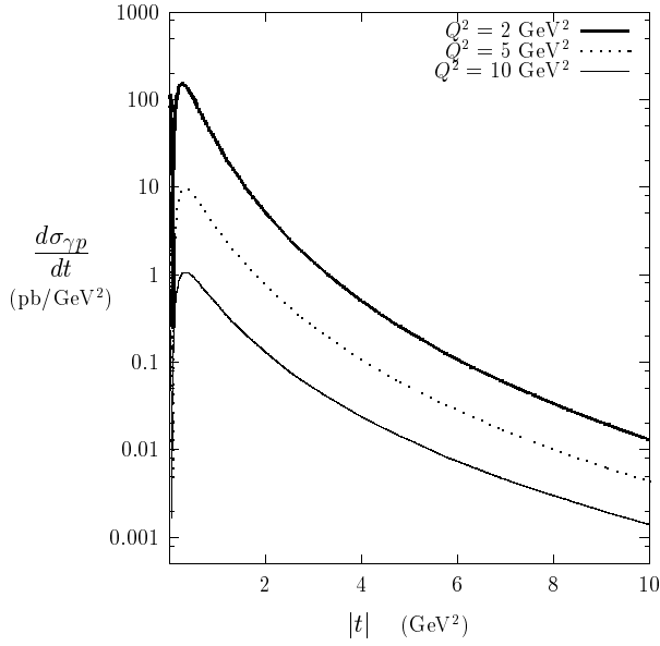
Fig. 7. The differential cross section for the process \gamma^* p \rightarrow \pi^0 p . The pion wave function has been approximated by the asymptotical form. The strong coupling constant has been evaluated with the scale \mu^2 = Q^2 + |t| and with \Lambda_{\text{QCD}}^{(4)} = 0.2 \text{ GeV}
