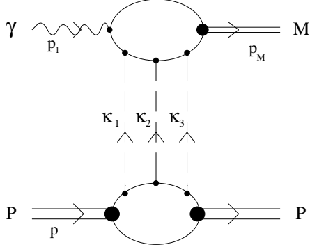
Fig. 1. The kinematics of elastic diffractive process \gamma^* p \rightarrow Mp
