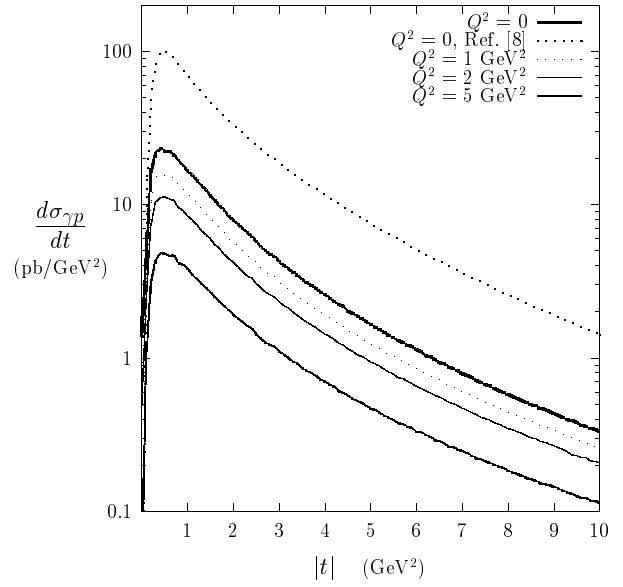
Fig. 3. Differential cross section for \gamma^* p \rightarrow \eta_C p . The strong coupling has been evaluated with the scale \mu^2 = m_c^2 and with \Lambda_{\text{QCD}}^{(4)} = 0.2 \text{ GeV}
