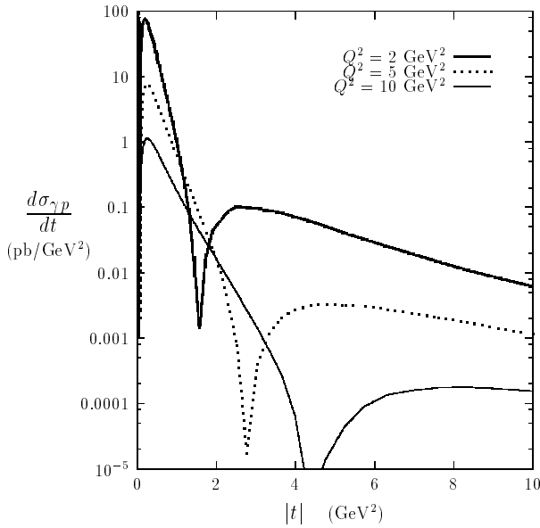
Fig. 8. The differential cross section for the process \gamma^* p \rightarrow a_2 p . The strong coupling has been evaluated with the scale \mu^2 = Q^2 + |t| and with \Lambda_{\text{QCD}}^{(4)} = 0.2 \text{ GeV}
