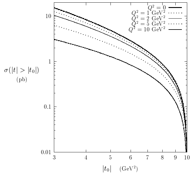
Fig. 6. Total cross section for the process \gamma^* p \rightarrow \eta_C X_p integrated over the region |t_0| < |t| . The integral over the quark densities in the proton has been restricted to x \geq 0.1
