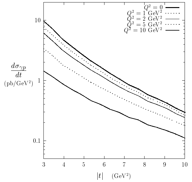
Fig. 5. Differential cross section for inelastic process \gamma^* p \rightarrow \eta_C X_p . The strong coupling has been evaluated with the scale \mu^2 = |t| and \Lambda_{\text{QCD}}^{(4)} = 0.2 \text{ GeV} . The integral over the quark densities in the proton has been restricted to x \geq 0.1
